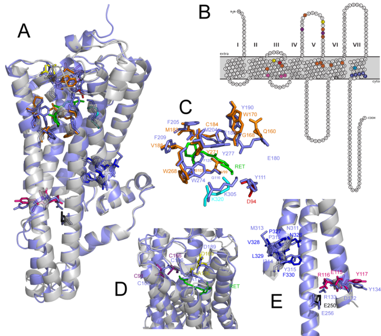
Figure 2.1: S. punctatus residues are colored according to function: orange (binding pocket residues), red (putative counterion), purple (disulfide bond), yellow (salt bridge), dark blue (NPxxY motif), and pink & black (ion lock). Light purple functional and backbone residues belong to T. pacificus , while grey backbone residues belong to S. punctatus . The ideal position of the 11- cis -retinal ligand, taken from the T. pacificus crystal structure, is shown in green. A) C\alpha backbone structural alignment of S. punctatus homology model and T. pacificus x-ray crystal structure. B) Topography plot of membrane spanning regions of S. punctatus homology model. C) Detail of S. punctatus binding pocket residues aligned with those of T. pacificus . D) Detail of S. punctatus disulfide bond (purple) and salt bridge (yellow) regions aligned with those of T. pacificus . The view is from the top (extracellular side) of the protein, into the 11- cis -retinal (green) binding pocket. E) Detail of S. punctatus ERY and NPxxY regions aligned with those of T. pacificus .
