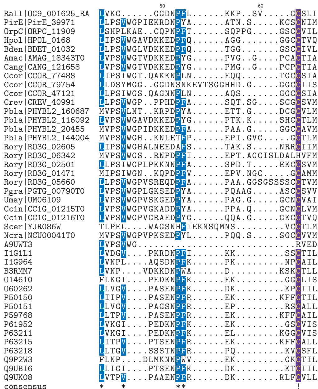
Figure 3.9: Multiple sequence alignment of C-termini of G \gamma proteins identified in fungi which possessed C-terminal pertussis (C[GAVLIP] 2 X) motifs aligned using T-coffee.
