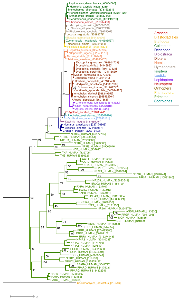
Figure 4.7: RAxML tree of select 20-hydroxyecdysone receptors from insects and Human nuclear receptors, and unique C. lativittatus protein sequences
