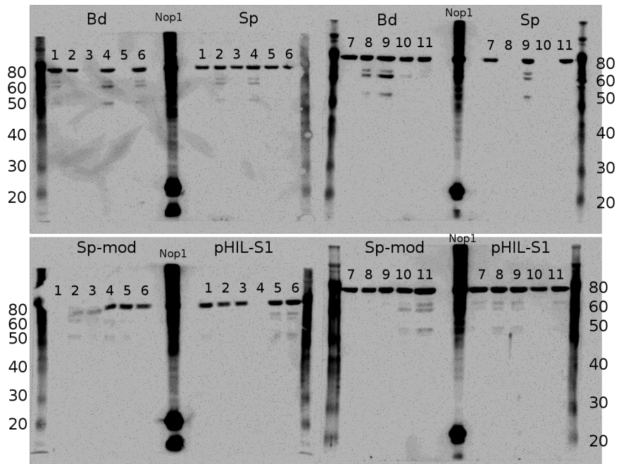
Figure 3.13: Western blots for heterologous Pichia pastoris expression of opsin constructs from Bd and sp , both native and missing lysine (" Sp-mod "). Expression of the expected Nop-1 protein from Neurospora crassa can be seen, and empty vector pHIL-S1 is included as a negative control.
