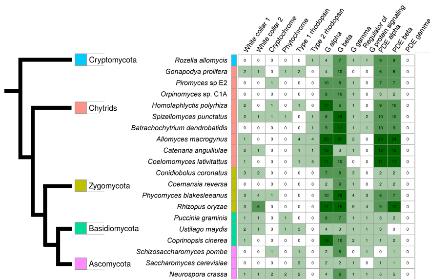
Figure 3.1: Photosensory protein distribution and G protein signaling pathway component distribution in representative subset of fungi.
