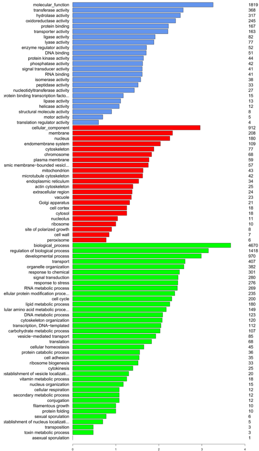
Figure 4.1: Distribution of Aspergillus GO-Slim terms in the C. lativitattus transcriptome.
