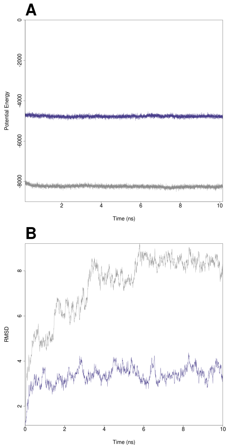
Figure 2.3: Overview plots of MD simulation runs of squid 2Z73 crystal structure with 11- cis -retinal (purple) and S. punctatus model with 9- cis -retinal (gray). A) Potential energy over course of simulation. During the simulation, both structures remain relatively stable. The S. punctatus structure has substantially lower potential energy than the squid structure. B) RMSd fits over course of simulation. The RMSd fit of the S. punctatus structural model increases much more rapidly than that of the squid structure, but ultimately reaches a plateau after approximately 6 ns.
