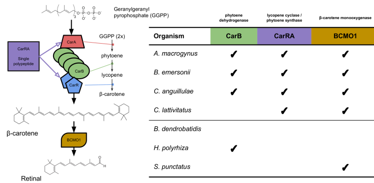
Figure 4.3: Presence and absence of \beta -carotene related proteins in species belonging to the Chytridiomycota and Blastocladiomycota.
