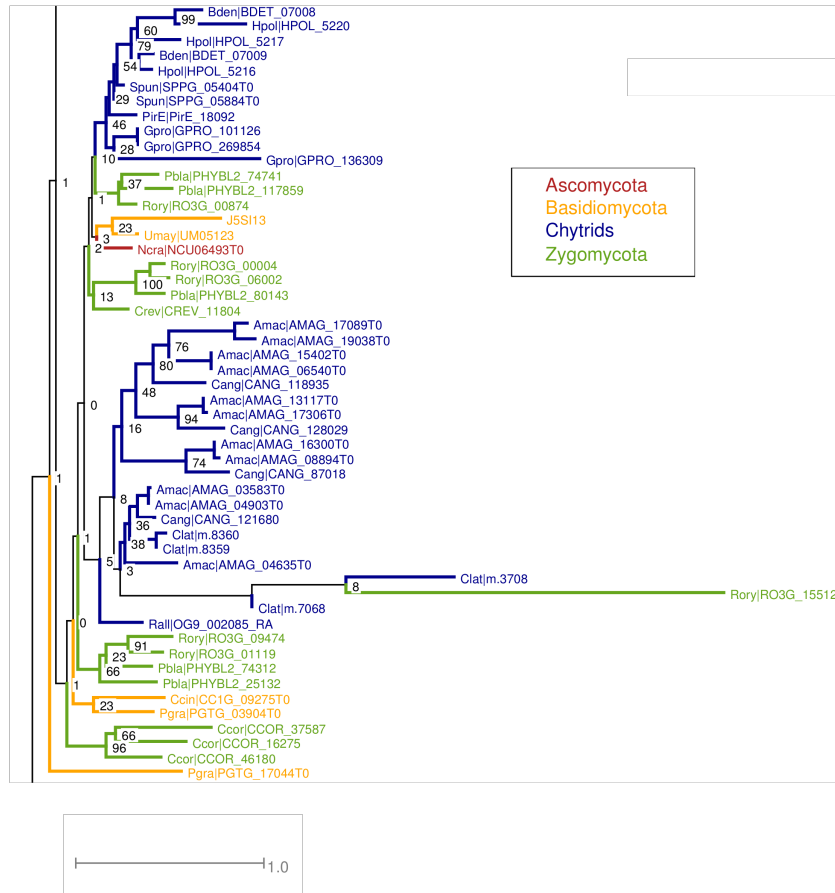
Figure 3.3: Maximum likelihood tree of identified G-α subunits in fungi (group I, as defined by inclusion of NCU06493)
