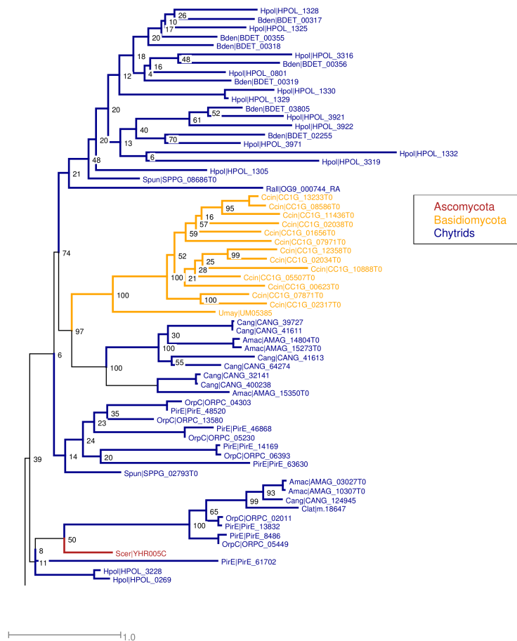
Figure 3.6: Maximum likelihood tree of identified G-α subunits in fungi (group IV, as defined by absence of N. crassa homologs and inclusion of UM05385 from Ustilago maydis )
