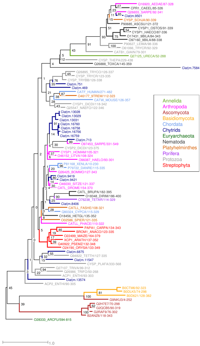
Figure 4.4: RAxML tree of select PF00112 seed sequences, unique C. lativitattus protein sequences, and sequences from Dikarya species.
