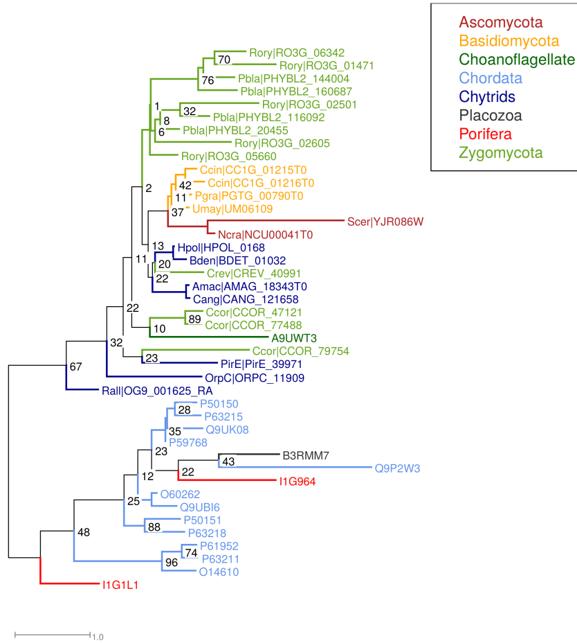
Figure 3.10: Maximum likelihood tree of identified G\gamma subunits in fungi and animal outgroups
