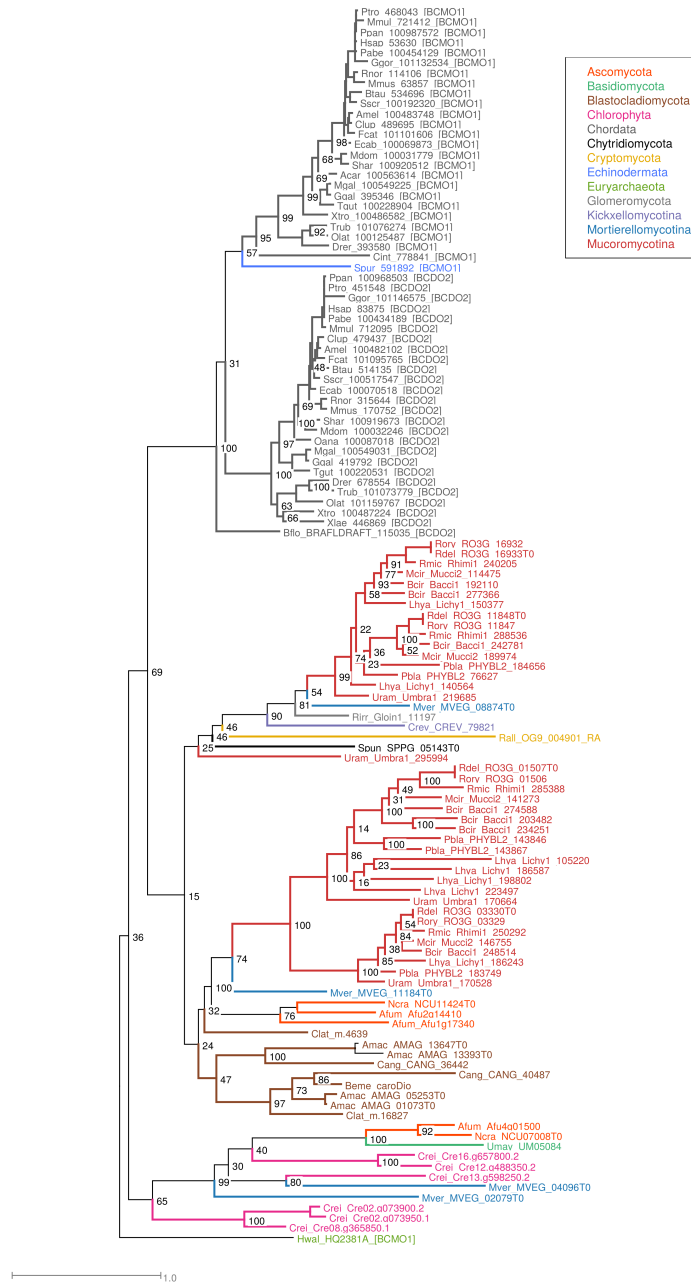
Figure 4.8: Phylogenetic history of BCMO1 homologs found in Fungi and Metazoan lineages using a maximum likelihood tree constructed with RAxML from identified BCMO1 fungal sequences and those from KEGG families.
