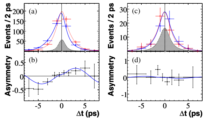
FIG. 2 (color online). Projections (see text) onto \Delta t for (a) \eta'K_S^0 and (c) \eta'K_L^0 of the data (points with error bars for B^0 tags in solid circles and \bar{B}^0 tags in empty rectangles), fit function (solid and dashed lines for B^0 and \bar{B}^0 tagged events, respectively), and background function (shaded regions). We show the asymmetry between B^0 and \bar{B}^0 tags for (b) \eta'K_S^0 and (d) \eta'K_L^0 ; the lines represent the fit functions.
