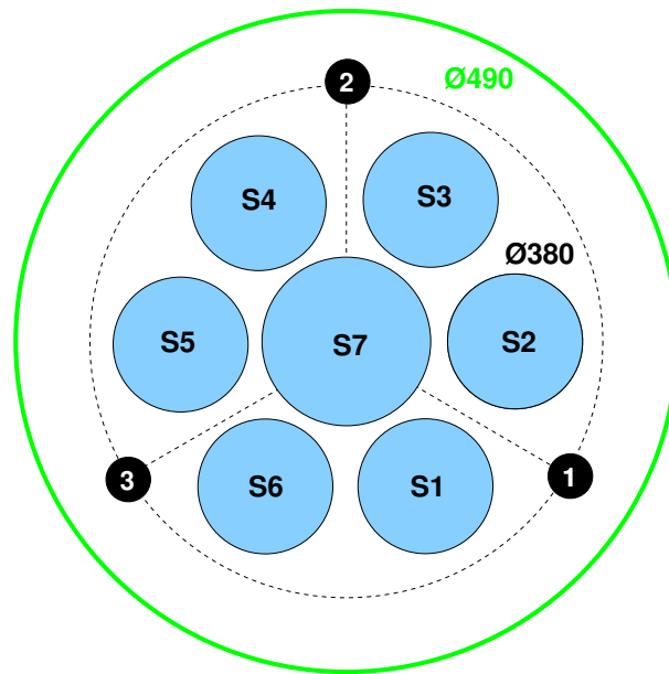
Fig. 32 View of the array from top. The positions of the three calibration sources (1, 2, 3) and the boundaries of the LAr veto system ( \text{\O}490 mm) are indicated. The surrounding radon shroud with a diameter of 750 mm [3] is not shown.
