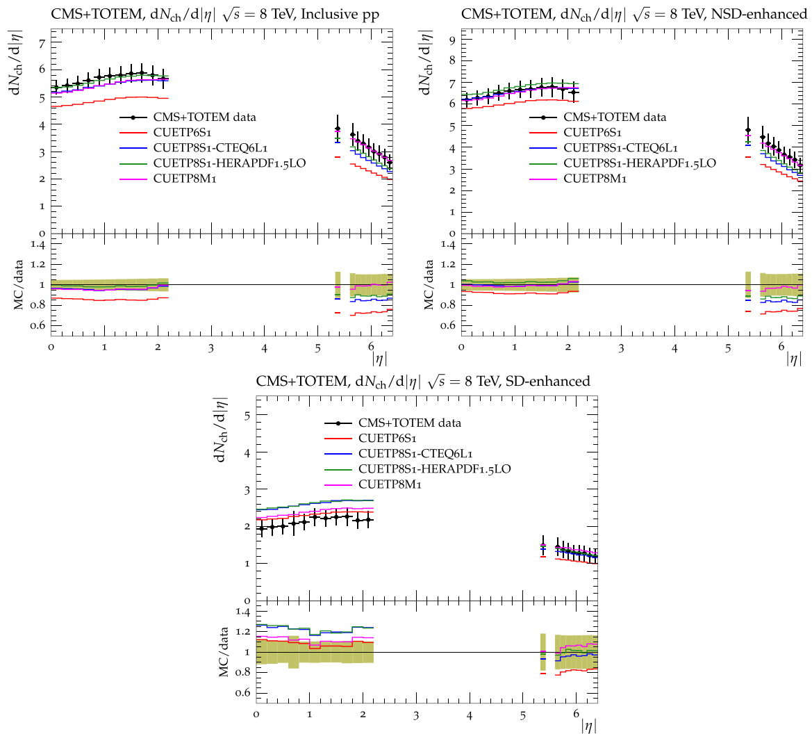
Fig. 13 Combined CMS and TOTEM data at \sqrt{s} = 8 TeV [50] for the charged-particle distribution dN_{ch}/d\eta , in inclusive inelastic (top left), NSD-enhanced (top right), and SD-enhanced (bottom) pp collisions. The data are compared to PYTHIA6 using CUETP6S1-CTEQ6L1, and to
