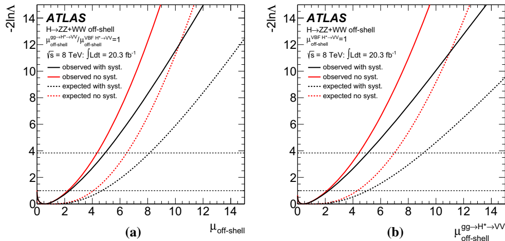
Fig. 9 Scan of the negative log-likelihood, -2\ln\Lambda , as a function of \mu_{\text{off-shell}} , for the combined ZZ and WW analyses. a Common signal strength \mu_{\text{off-shell}} applied to both the gg \rightarrow H^* and VBF processes. The ratio of the gg \rightarrow H^* and VBF processes is assumed to be as in the SM. b Signal strength \mu_{\text{off-shell}}^{gg \rightarrow H^* \rightarrow VV} for the gg \rightarrow H^* \rightarrow VV process. The production rate for the VBF
