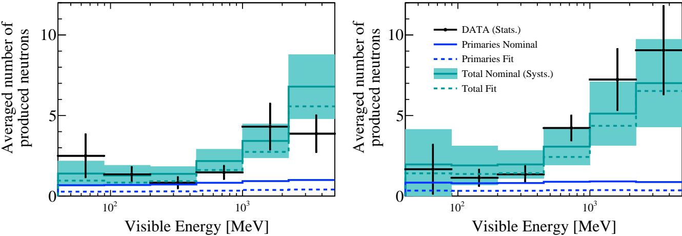
FIG. 18. Number of produced neutrons vs visible energy for CCQE (left) and non-CCQE (right) selections before and after \chi^2 fit to neutron components. This combines both phases.
