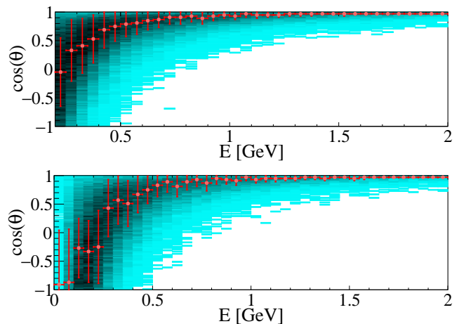
FIG. 5. Angle of produced lepton \cos\theta_l vs lepton energy in a CCQE neutrino interaction for muons (top) and electrons (bottom). The red dots show the mode of the \cos\theta distribution at each energy bin with the 1\sigma uncertainty.
